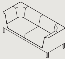
TWO SEATER LOUNGE W 1900 D 770 H 725 S 400
