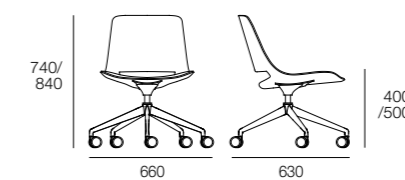
Palm aluminium 5-way castor
